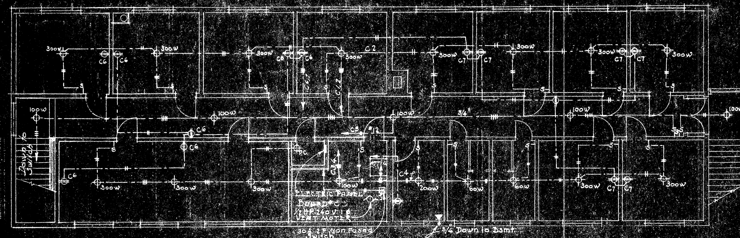
SECOND FLOOR PLAN ELECTRICAL SCALE 1/8" = 1'-0"
